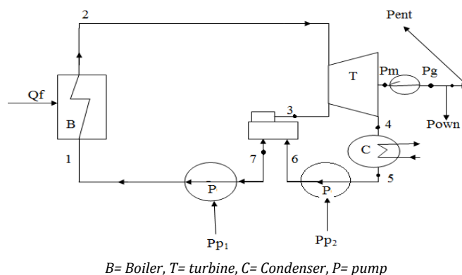
Figure 2: Schematic of Power Plant
